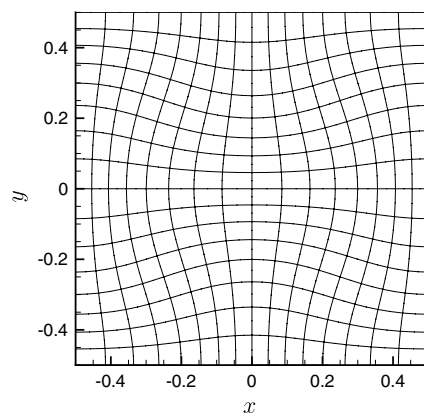
Fig. 6. The deformed solid mesh in the solid-only convergence test.
