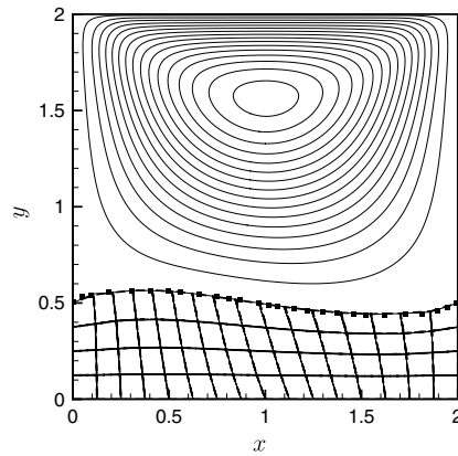
Fig. 9. The steady state of the deformation of an elastic wall driven by flow. The \blacksquare shows the interface position of Dunne [8]. The solid mesh is shown both for the present force-projection method — and an Arbitrary Lagrangian–Eulerian method ---.
